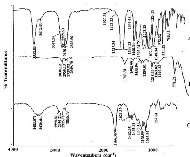
Figure 4. FT-IR spectra of SIM (A), PLGA (B), and SIM-loaded PLGA NPs.
